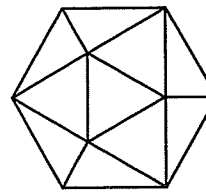
Icosahedron
