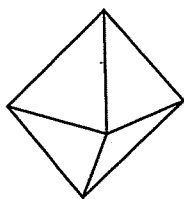
Octahedron
